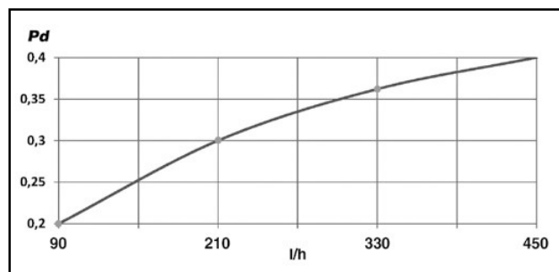
DN 20 Model
