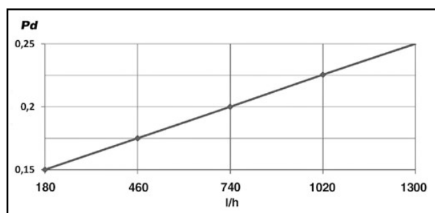
DN 20 Model
